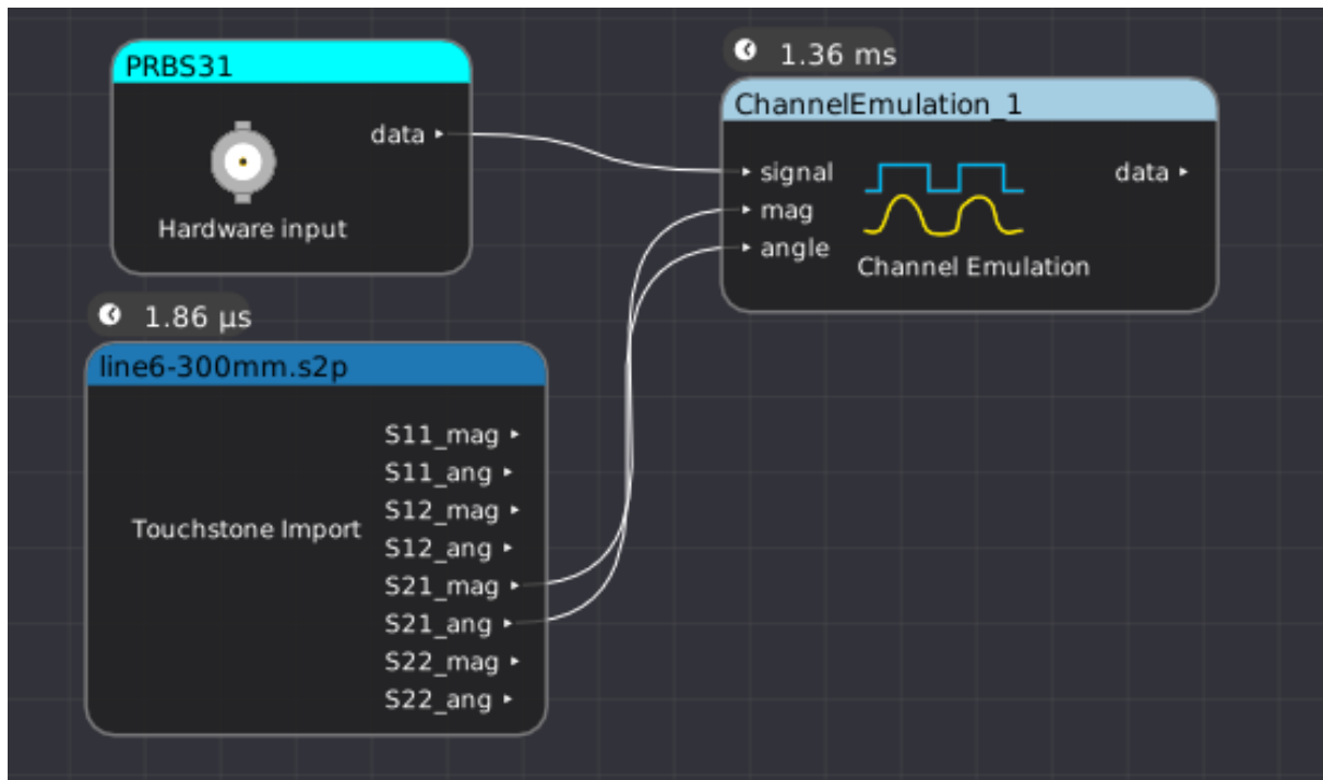
Figure 26.41: Example filter graph showing usage of channel emulation filter
