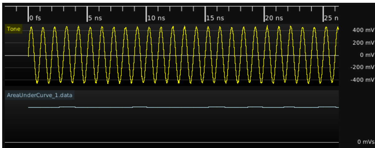
Figure 26.22: Absolute area per cycle measurement. In this mode, the filter outputs \int_{t1}^{t2} |x| at each zero crossing bounded interval, so we get \int_0^{2\pi} |\sin(x)| = 4 (plus measurement noise).
