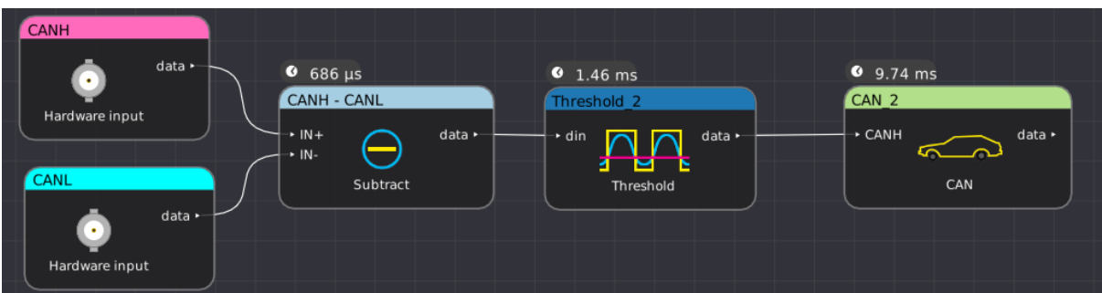
Figure 26.36: Example filter graph showing usage of CAN bus decode
