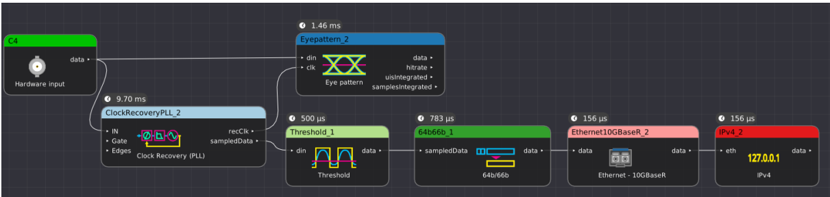
Figure 26.6: Example filter graph using 64b/66b to decode a 10GbE signal
