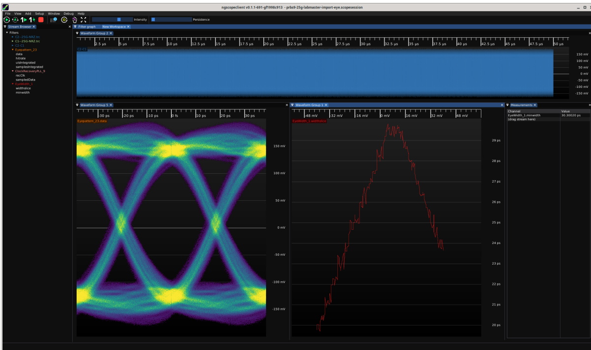
Figure 26.135: Example of measuring width of an eye pattern
