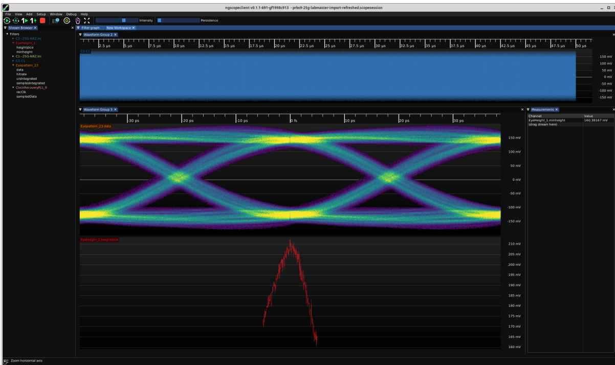
Figure 26.127: Example of measuring height of an eye pattern
