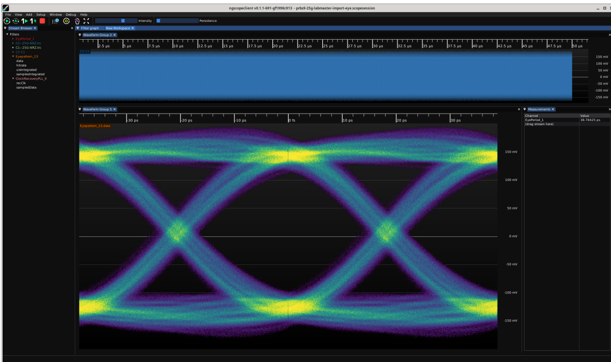
Figure 26.133: Example of measuring period of an eye pattern
