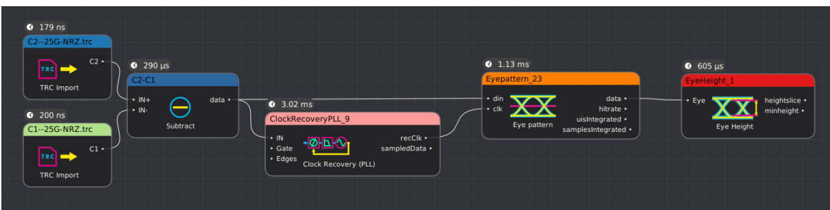
Figure 26.128: Example filter graph measuring height of an eye pattern
