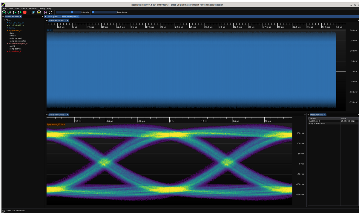
Figure 26.125: Example of measuring bit rate of an eye pattern
